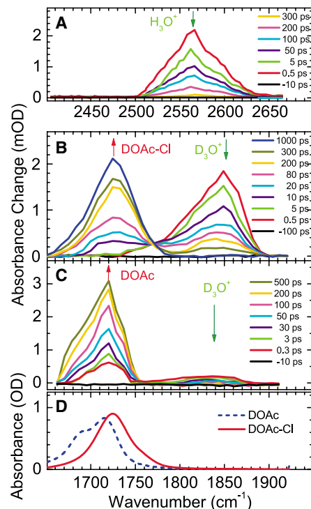
Fig. 2. Transient response of the hydronium O-H stretching band at 2570\text{ cm}^{-1} measured with 1\text{ M } ^-\text{OAc-Cl} in \text{H}_2\text{O} (A), the C=O stretching band of DOAc-Cl at 1725\text{ cm}^{-1} , and the hydronium O-D stretching band at 1850\text{ cm}^{-1} for 1\text{ M } ^-\text{OAc-Cl} in \text{D}_2\text{O} (B). For comparison, the transient response of a solution with 1\text{ M } ^-\text{OAc} in \text{D}_2\text{O} is shown in (C), as well as the steady-state spectra of DOAc and DOAc-Cl also measured in \text{D}_2\text{O} (D).
